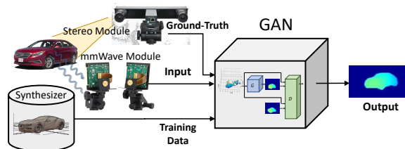
Figure 2: HawkEye’s System Overview.
